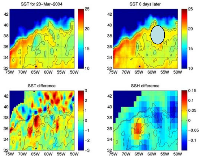
Cold core ring: March 2004
